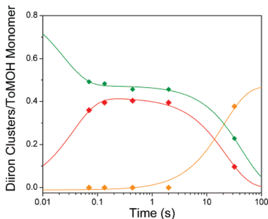
Figure 3. Speciation plot for reaction of diiron(II) ToMOH:2ToMOD with dioxygen. Reduced diiron(II) protein (green diamonds) reacts with dioxygen at \sim 26 s ^{-1} to form a diiron(III) transient species (red diamonds). Only \sim 45\% of diiron(II) clusters give rise to this intermediate. The diiron(III) transient subsequently decays to the oxidized resting state (orange diamonds) at \sim 0.045 s ^{-1} . The unreacted diiron(II) centers decay slowly at 0.02 s ^{-1} to generate several ill-defined ferric species, the production of which is not depicted. Solid lines are one- or two-exponential fits to the data.
